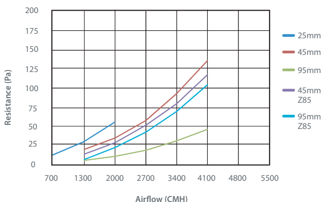
Filtro Carb Z - Airflow vs. Initial Resistance
