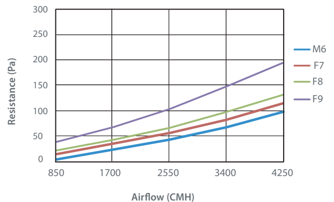
Filtro Cell SV - Airflow vs. Initial Resistance
