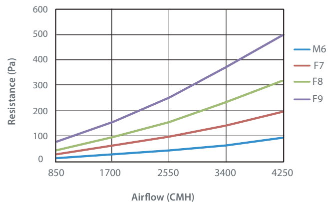
Filtro Cell V - Airflow vs. Initial Resistance
